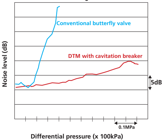
Noise comparison in valve opening 70 degree
